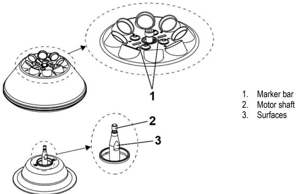
Figure 15: Rotor installation and removal
