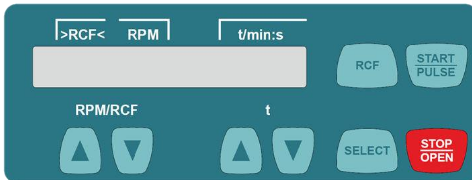
Figure 2: Control panel
