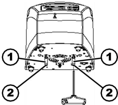
Figure 13: Transport lock
